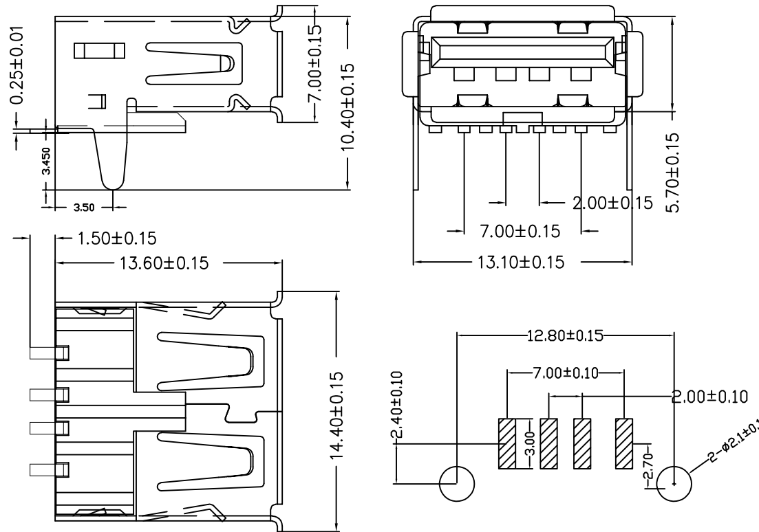
PCB LAYOUT
