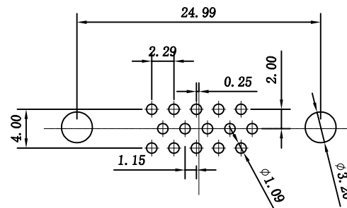
RECOMMENDED PCB LAYOUT (PRINTED SIDE, TOLERANCE ±0.05)
