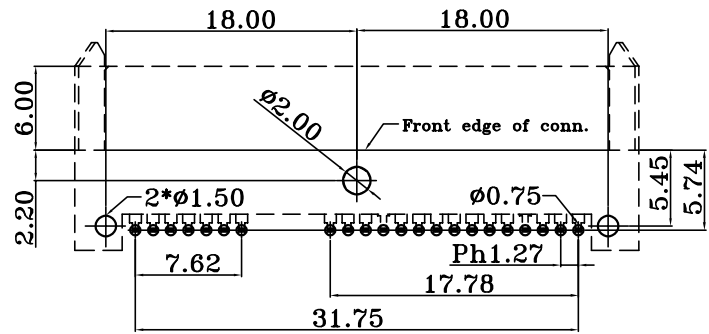
RECOMMEND PCB LAYOUT (T=1.6) PCB TOLERANCE:±0.05
